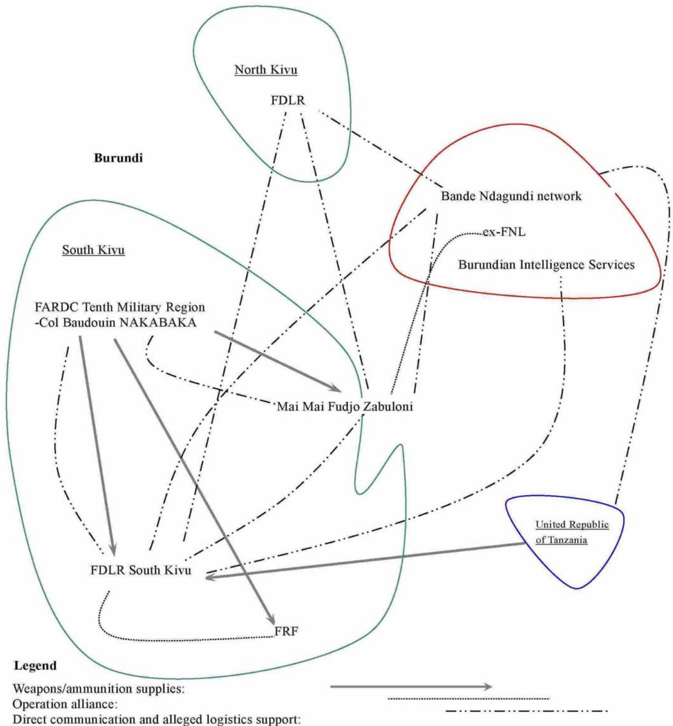
Diagram showing supply and support networks to armed groups in South Kivu
