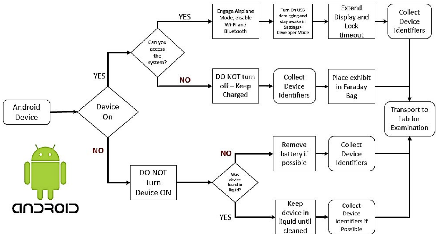
Figure 6: Flowchart for Android device evidence acquisition procedure
